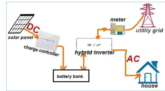
Hybrid inverter
