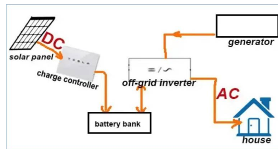
Off-grid inverter
