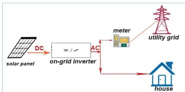
On-grid inverter
