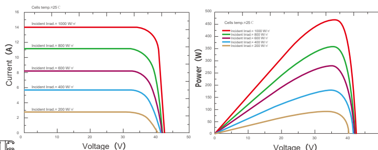
Current-Voltage & Power-Voltage Curves (SKT480 M10-120D4)
